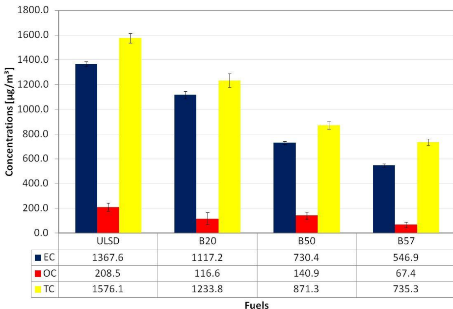
Effects of Fuels on EC, OC, TC Concentrations (TOT-EGA)
