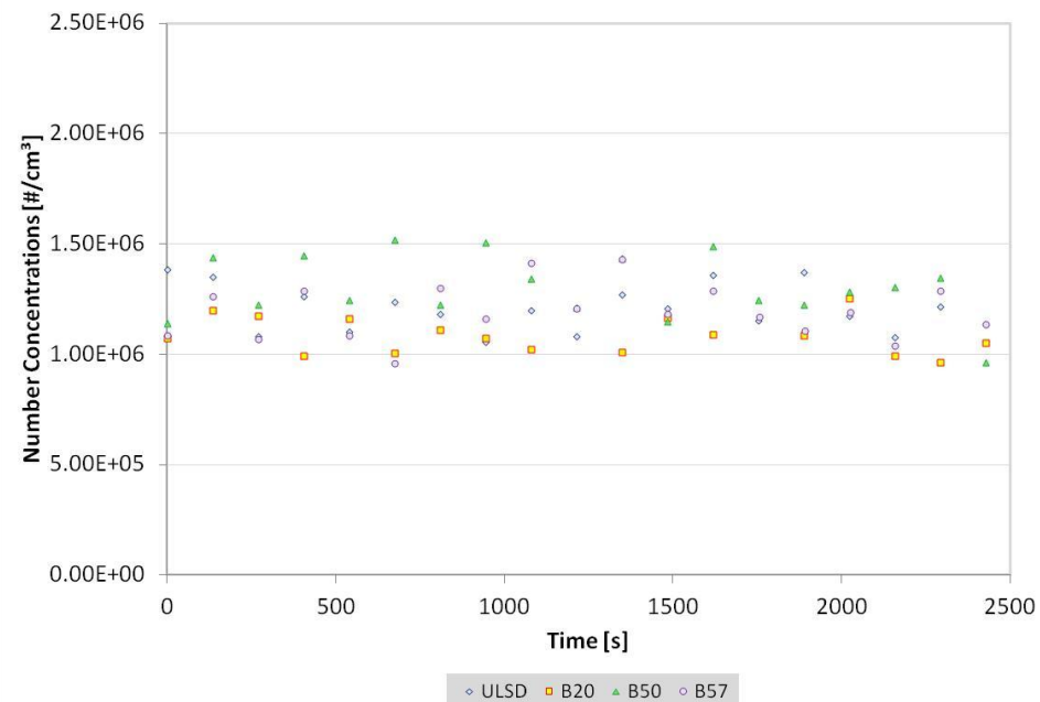
Number Concentrations of Aerosols Measured by SMPS at MS
