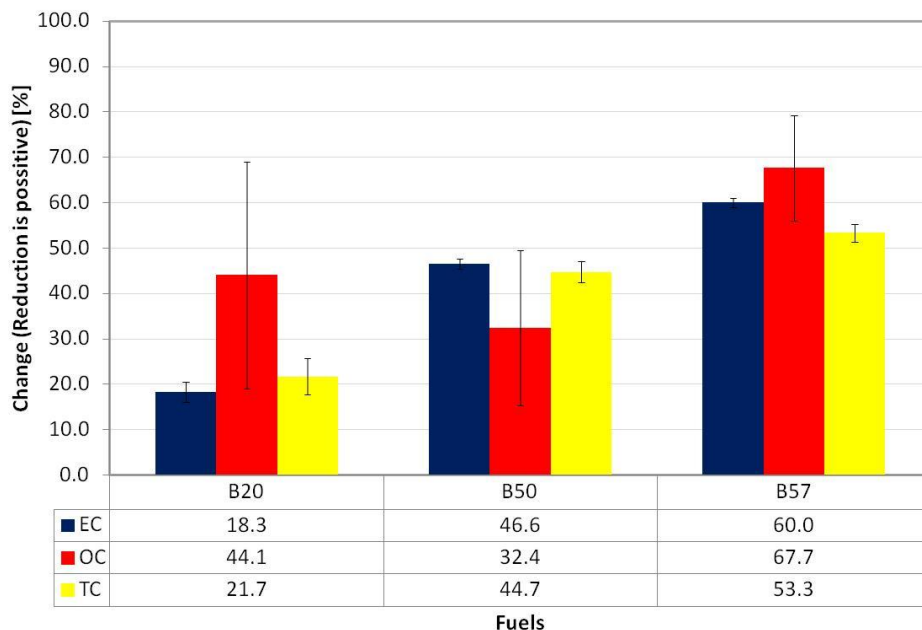
Changes in EC, OC, and TC Concentrations (TOT-EGA)
