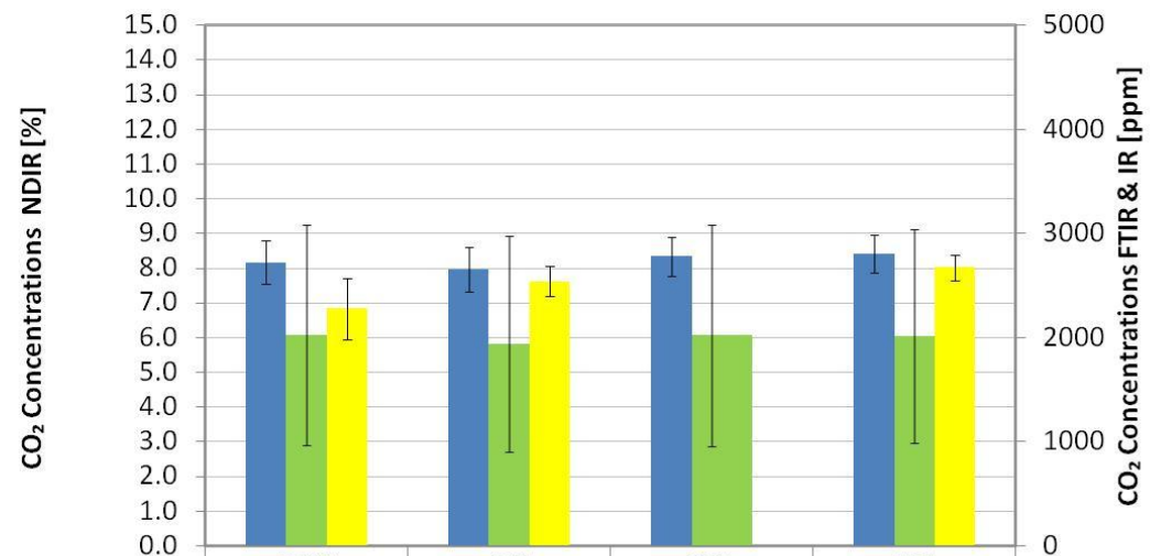
Average CO 2wet Concentrations in Tailpipe (NDIR) and in Ambient Air at MS (FTIR & IR)
