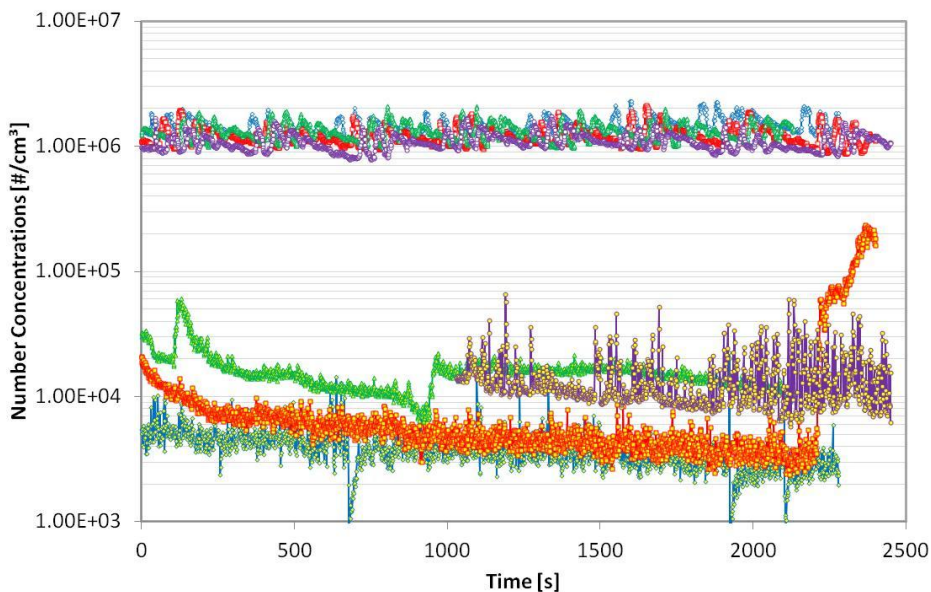
Number Concentrations of Aerosols Measured by FMPSs at MS & BS
