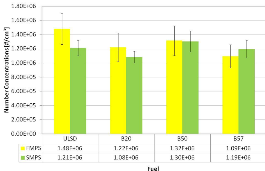
Effects of Fuel Formulations on Average Number Concentrations of Aerosols at MS
