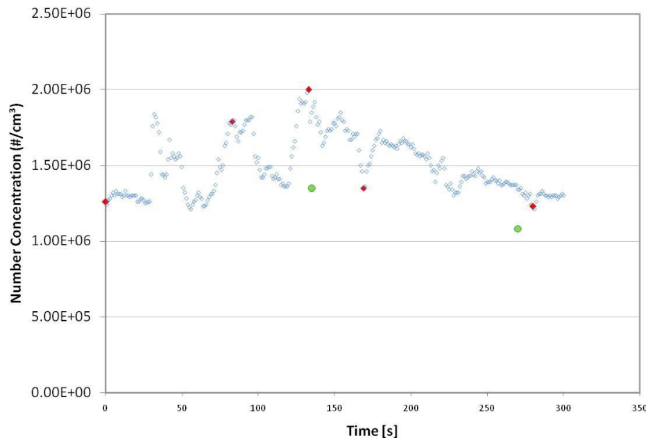
TC Concentrations FMPS and SMPS (ULSD, Cycle 2)
