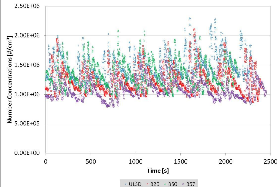
Number Concentrations of Aerosols Measured by FMPS at MS
