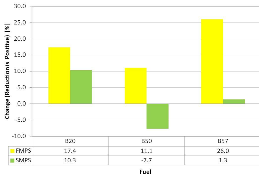
Effects of Fuel Formulations on Average Number Concentrations of Aerosols at MS
