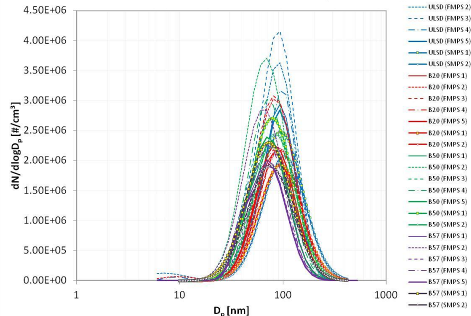
Effects of Fuel Formulation on Size Distributions (FMPS & SMPS)
