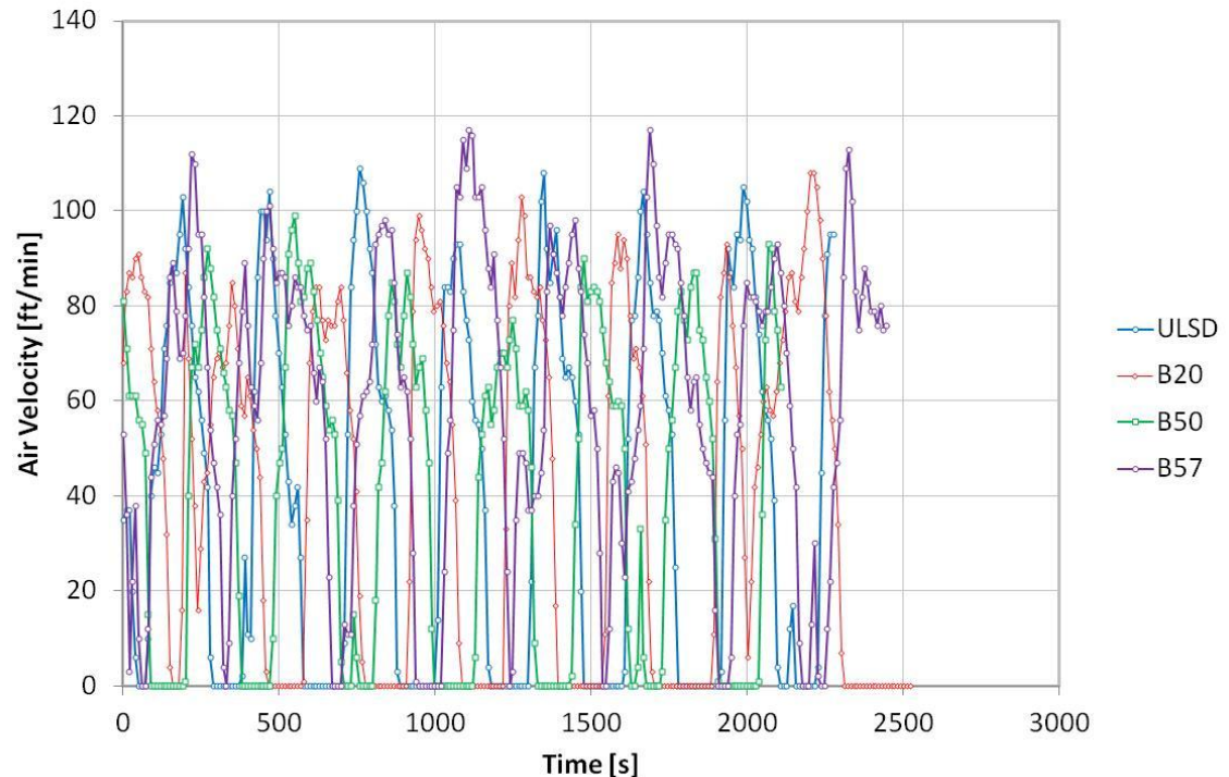
Air Velocity Measured at Centrally Located Single Point at MS During Fuel Tests
