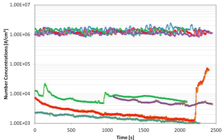
Number Concentrations of Aerosols Measured by CPCs at MS & BS
